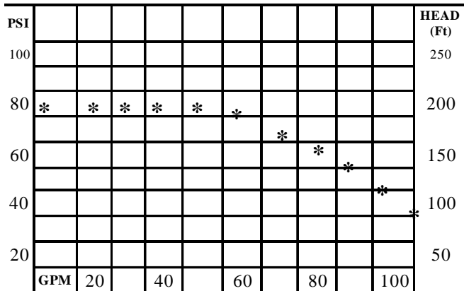
6.5 HP PUMP CURVE
